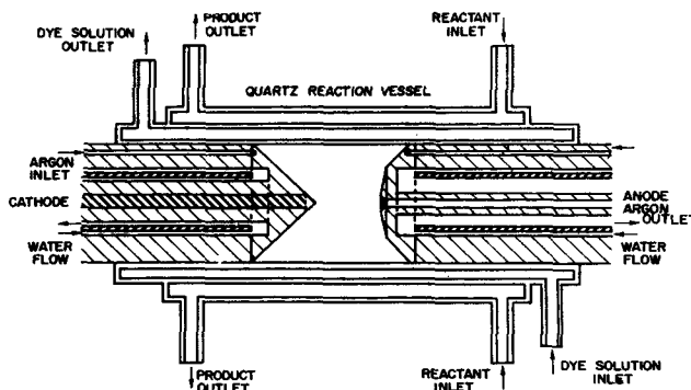
Fig. 2. Schematic diagram of photochemical reaction system.
